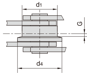
带F型带肩滚子 with F flanged rollers type
