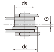
带F型带肩滚子 with F flanged rollers type
